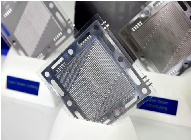
Figure 1: Laser-machined bipolar plates: Precise technology for improved corrosion resistance and efficiency in fuel-cell production. © Fraunhofer ILT, Aachen, Germany.
